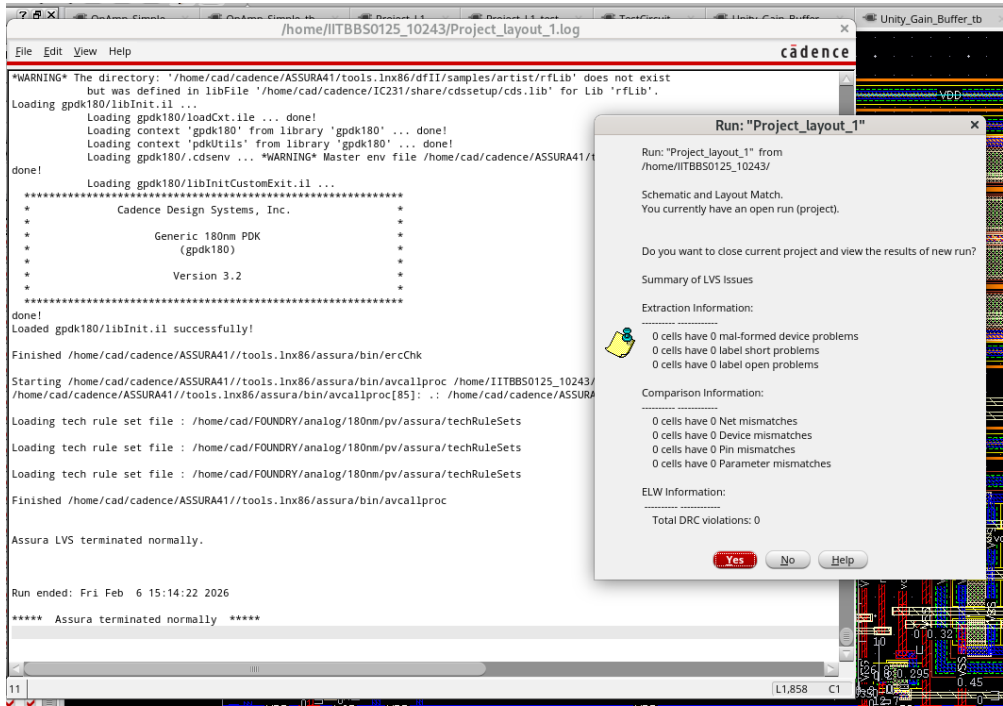
LVS Status: Clean
